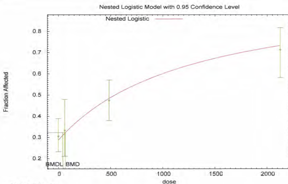
Figure 5-2 Fit of the nested logistic (NLogistic) model– to the incidence of extra cervical rib in fetal mice versus C max adjusted for background of methanol in blood from a GD6-GD15 inhalation study in mice. The BMD is estimated based on a BMR of 0.05 extra risk.
